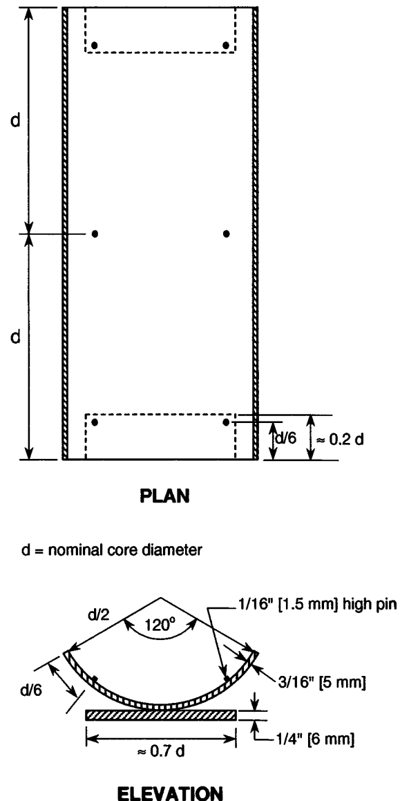
FIG. 1 Suitable Capping Device for Splitting Tensile Strength Test
